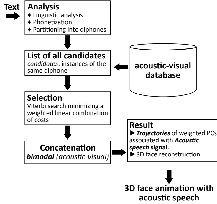
FIGURE 3.5 – Bimodal Text to speech synthesis processing.
