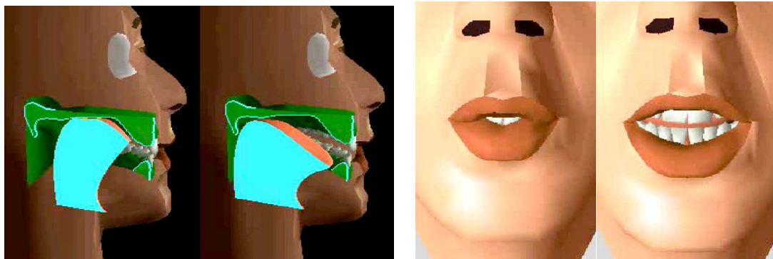
FIGURE 4.2 – (Left) Illustration of the internal articulatory processes of /k/ and /q/. (Right) Frontal view of /ly/ and /li/ at the point of maximum articulation of the vowel.
